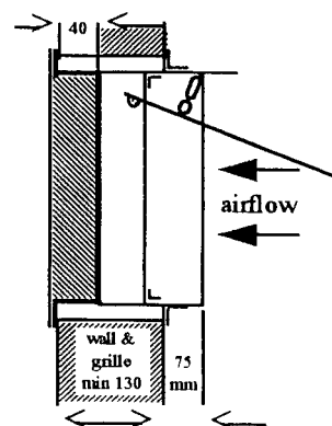
Wall Mounting with Grille
